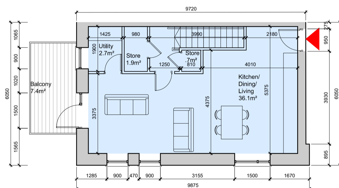
Unit Type H6.4.1 Scale 1:100 @ A1
