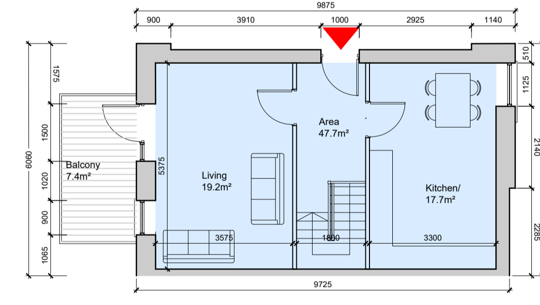
Unit Type H6.4.2 Scale 1:100 @ A1
