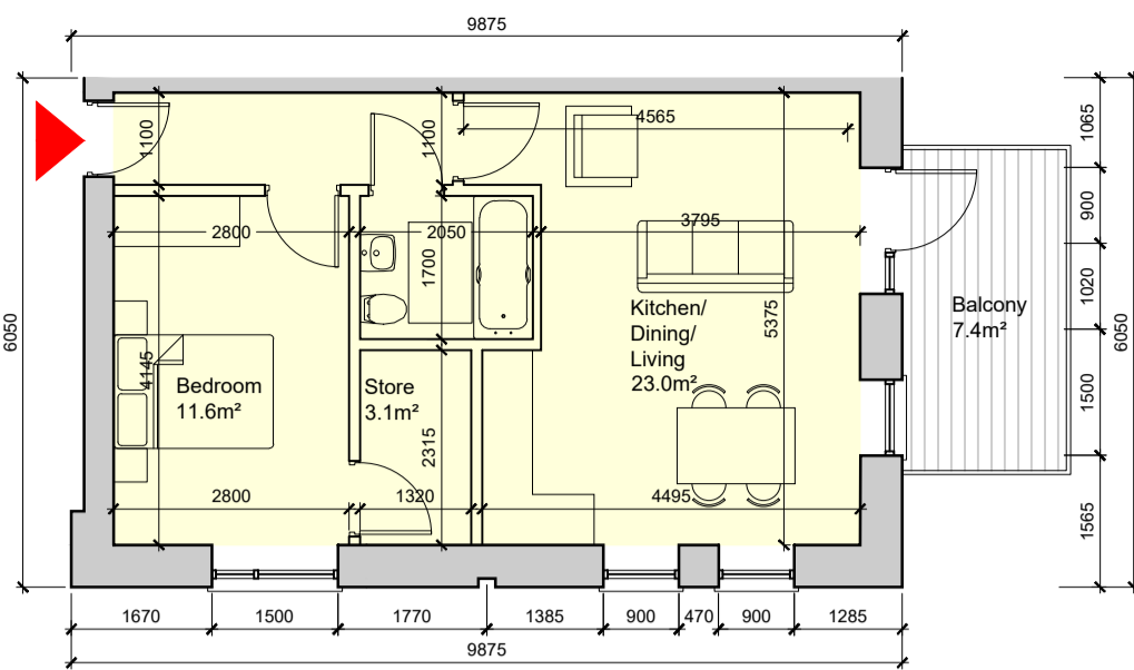
Unit Type H8.4.1 Scale 1:100 @ A1
