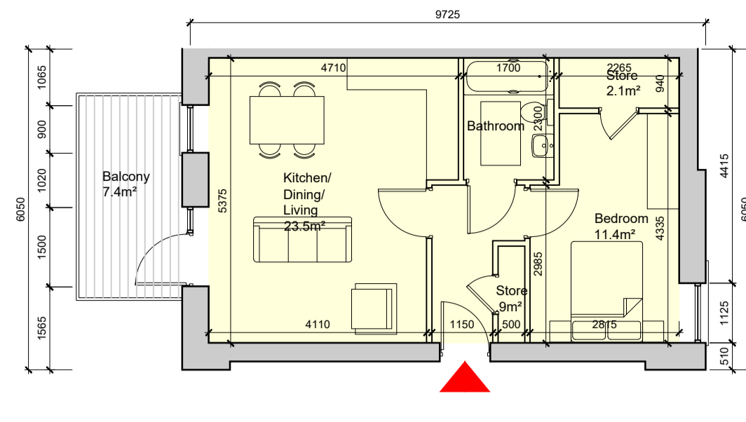
Unit Type H8.4.2 Scale 1:100 @ A1
